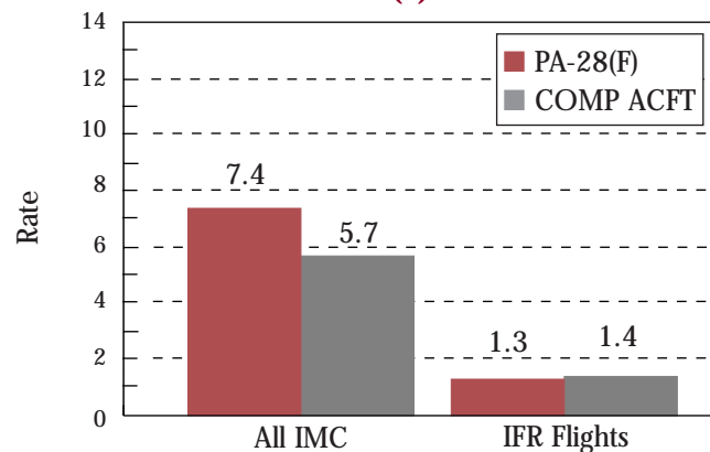
Figure 6. IMC Accidents Per 100,000 IMC Hours PA-28(F)
